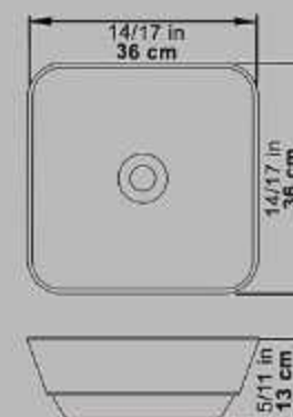
Top Counter Basin Square SIMPLE Without Tap Hole Built in
