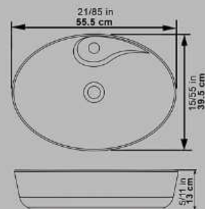
Top Counter Basin Ellipse TERMEH With Tap Hole Built in
