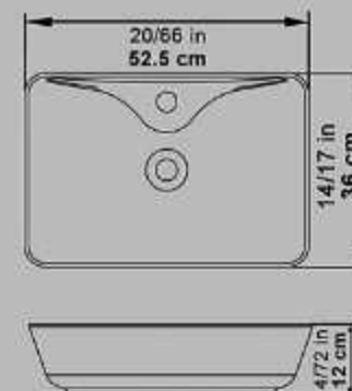
Top Counter Basin Rectangle HOMA With Tap Hole Built in
